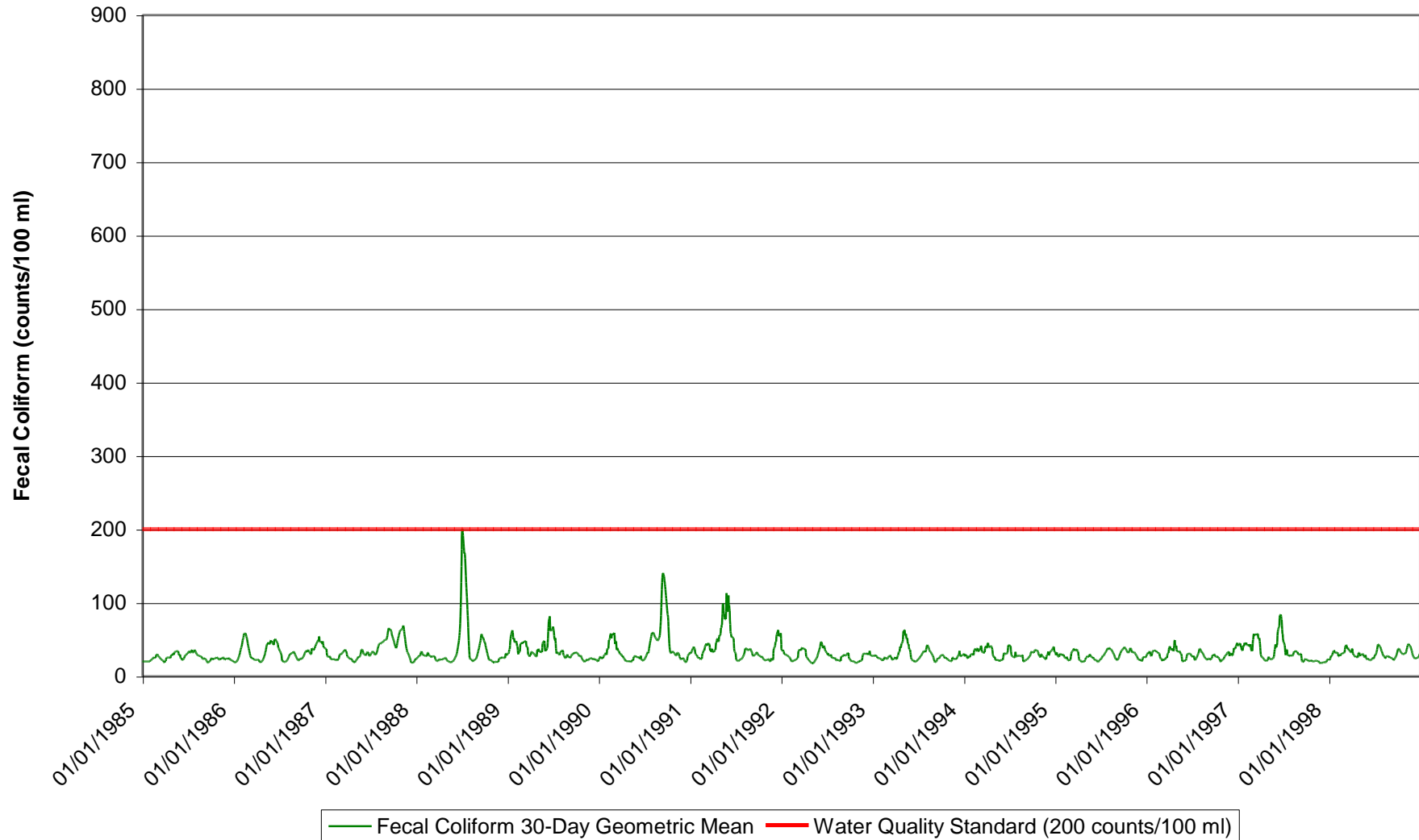
Graph A-4 Modeled Fecal Coliform Concentrations After Application of TMDL Scenario for Reach 08010207006
