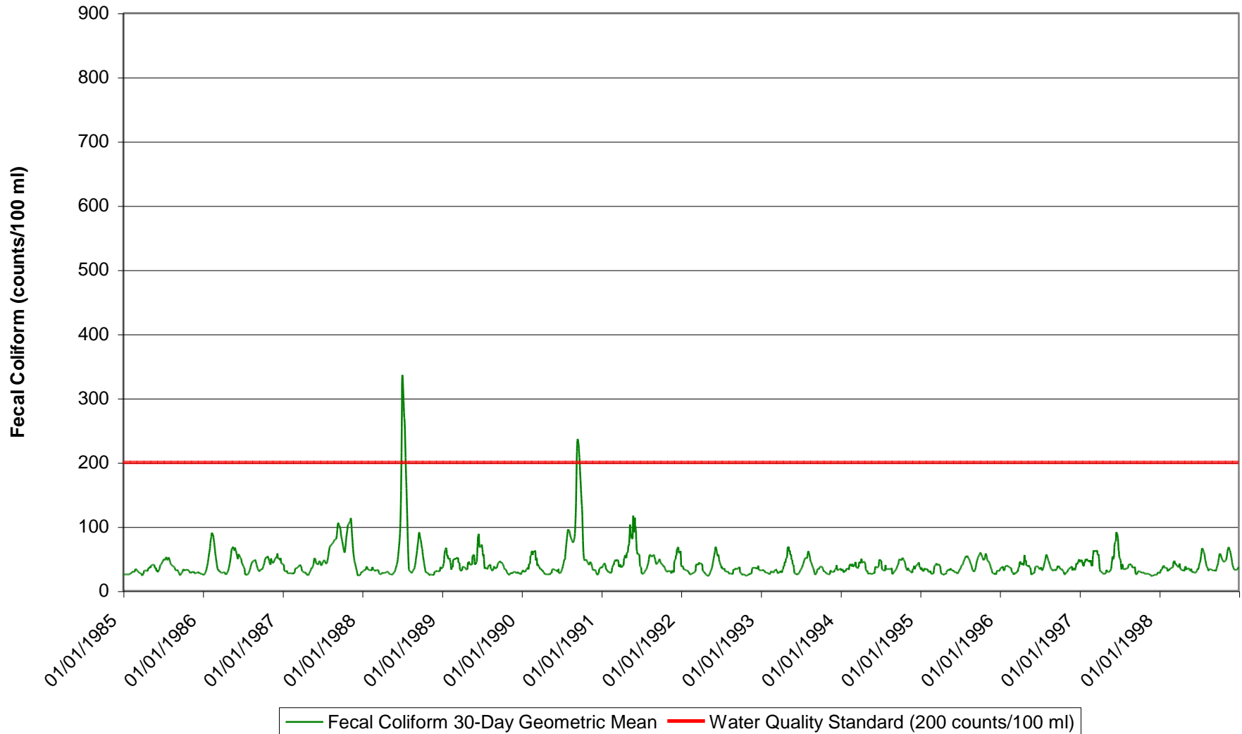
Graph A-3 Modeled Fecal Coliform Concentrations Under Existing Conditions for Reach 08010207006
