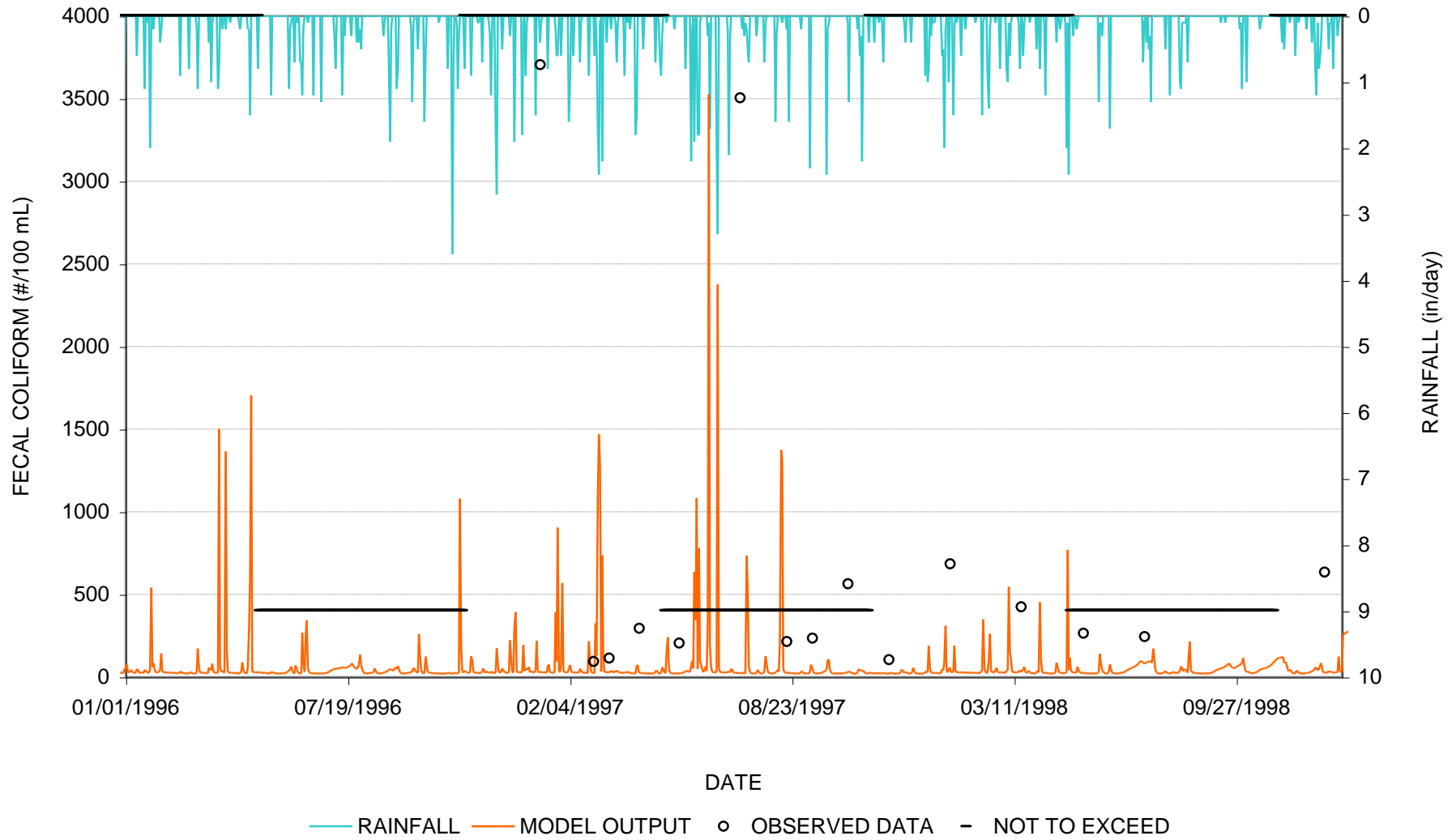
Graph A-2 Water Quality Calibration Plot for Reach 08010207006 and DEQ Ambient Monitoring Station 07029270
