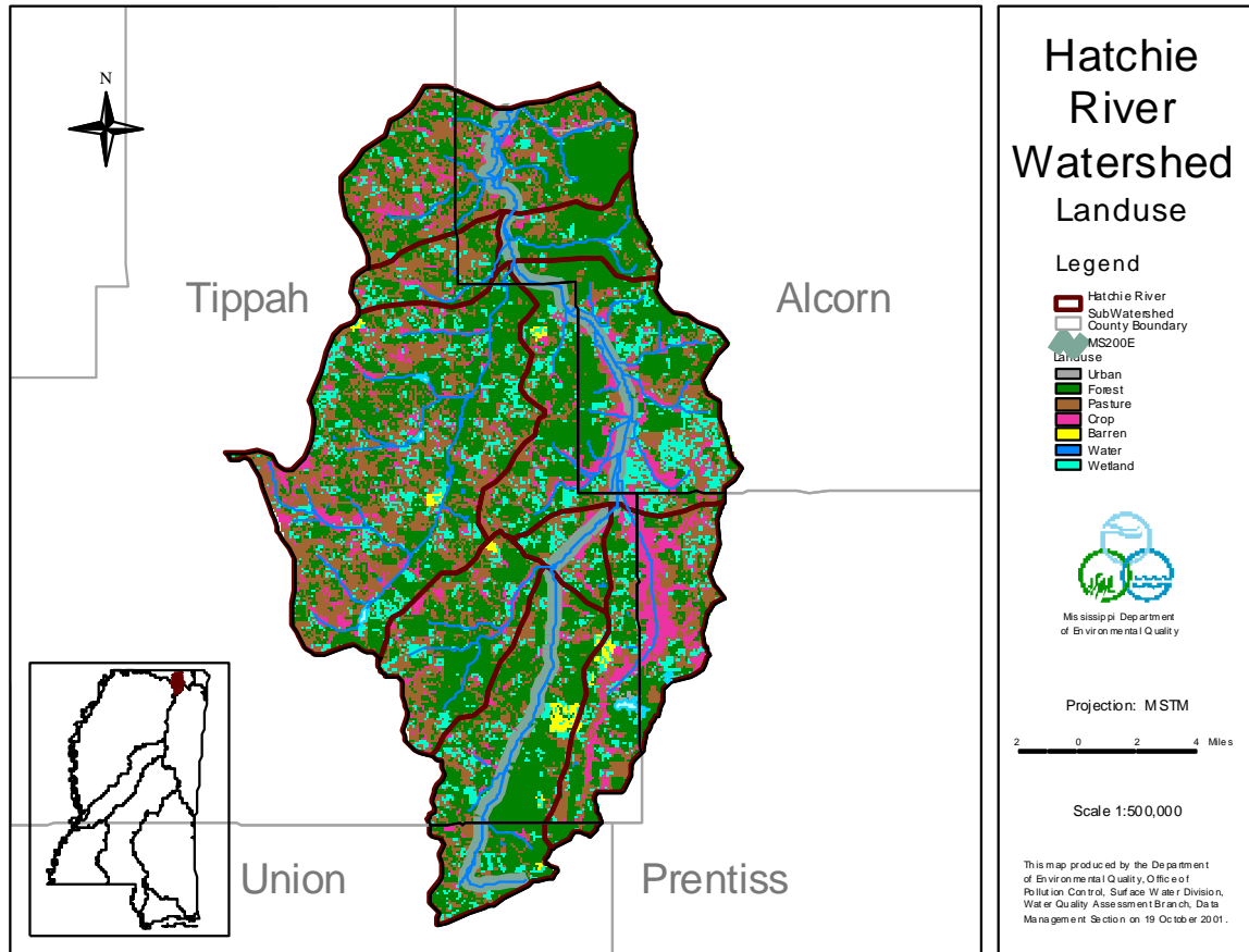
Figure 3.2 Landuse Distribution
